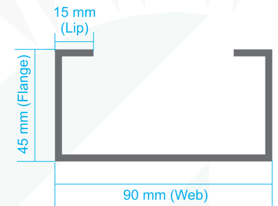
'C' Channel
