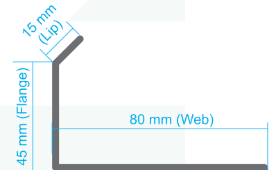
'Z' Channel
